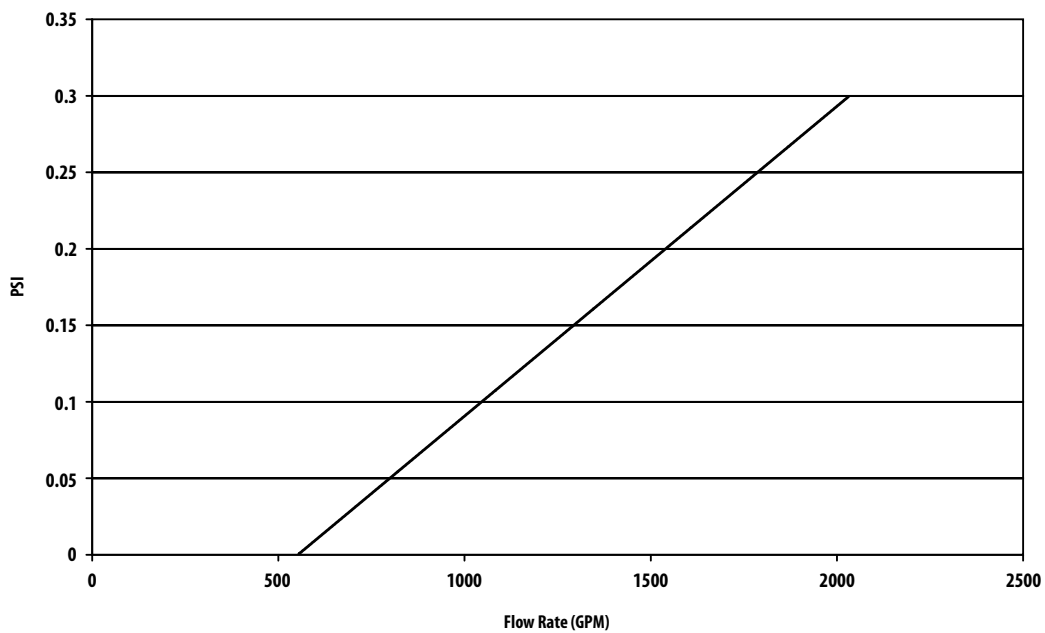
Head Loss Curve - 24" x 24"
