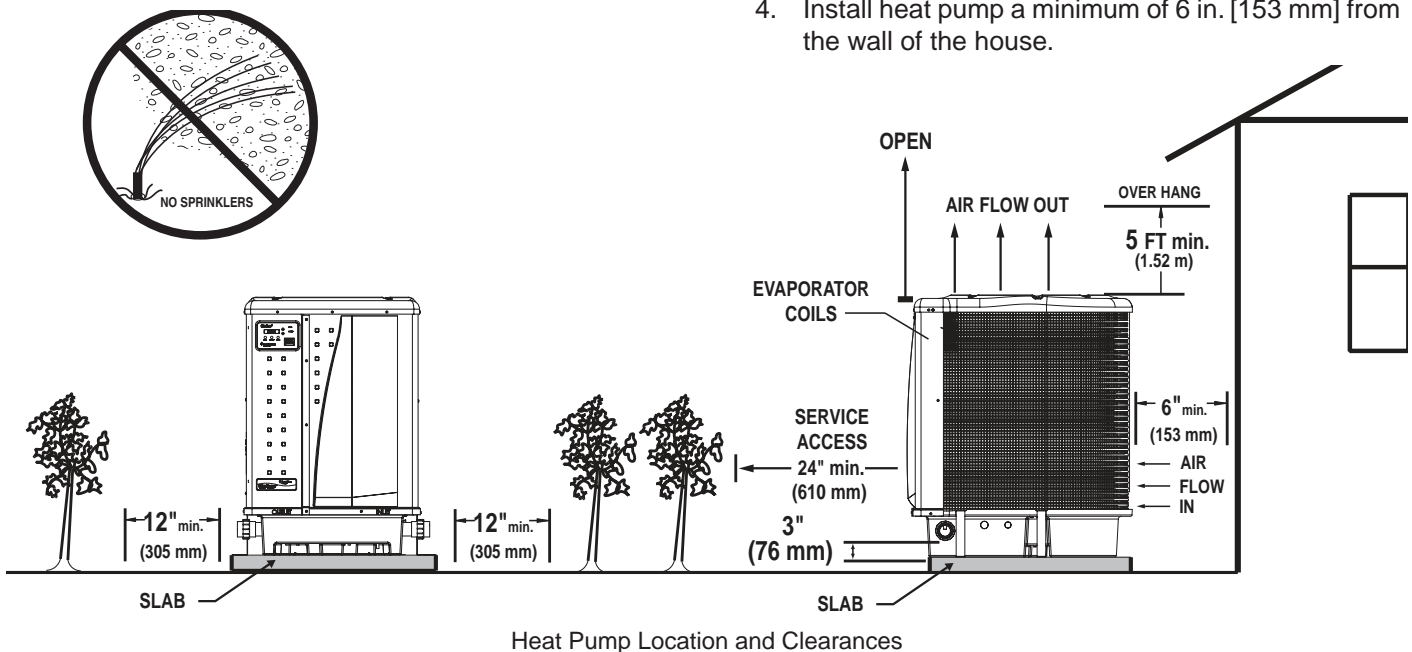
Heat Pump Location and Clearances
