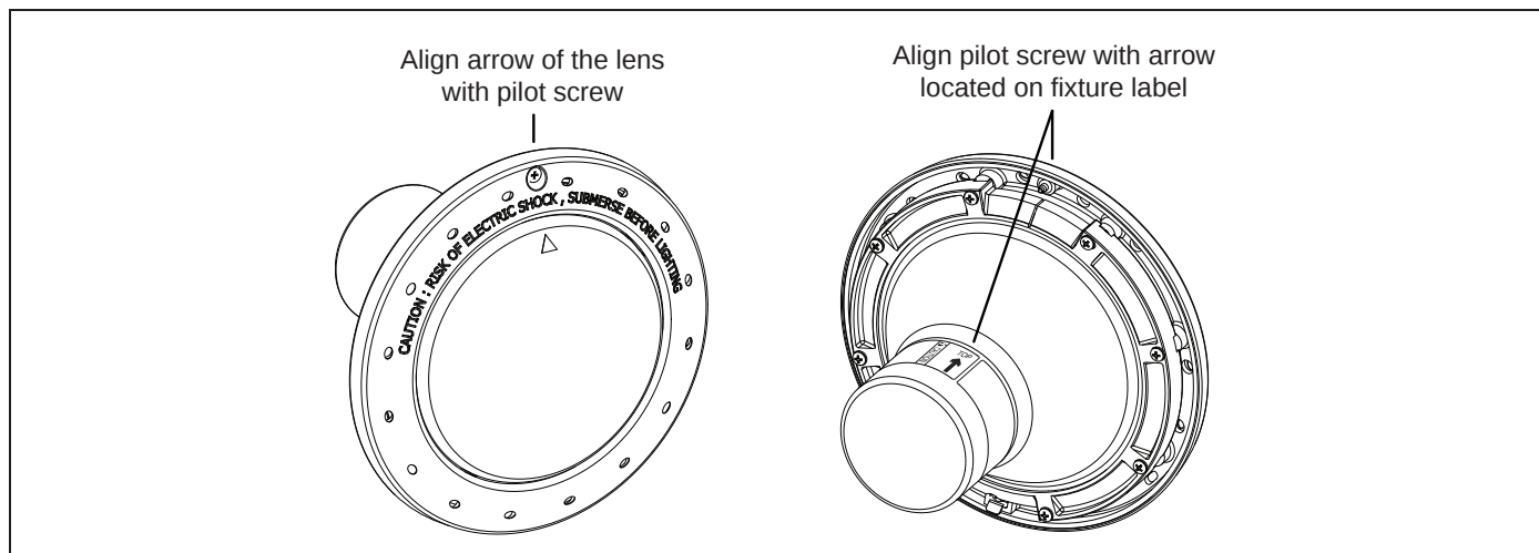
Figure 2. Alignment of the Lens, Face Ring, Housing and Clamps for Pool White Lights
