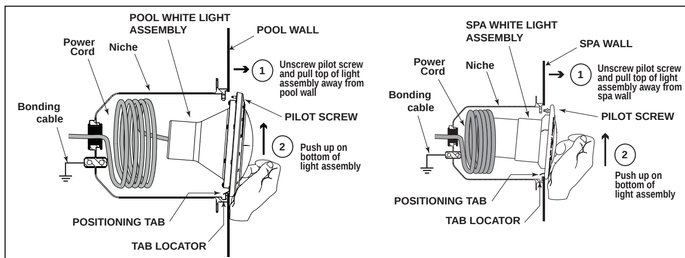
Figure 1. Removing the Pool and Spa White Light Assembly for Lamp Replacement
