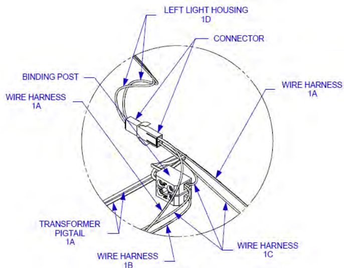
Detail G
