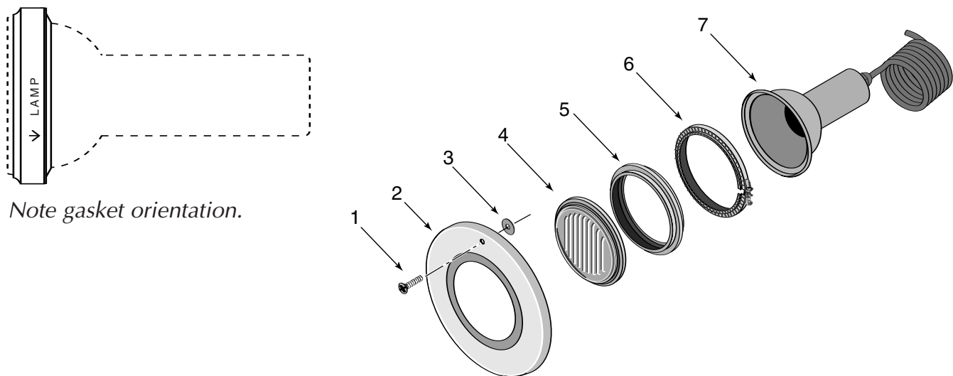
Figure 2 – SunLite® LTC Lamp Exploded View
