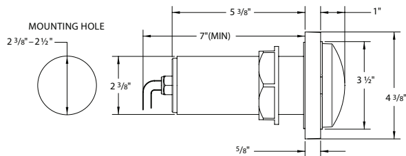
OVERALL DIMENSIONS
