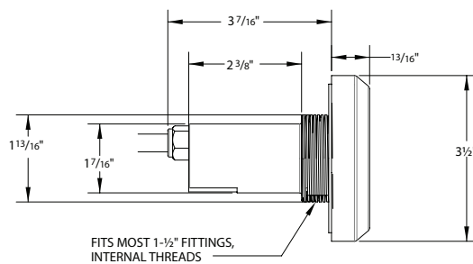
OVERALL DIMENSIONS
