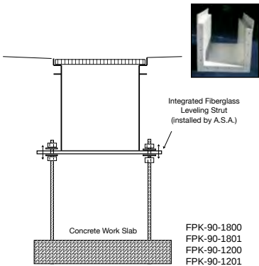
The preferred modular fiberglass gutter system for rimflow pools, zero entry, beach entry and spray deck designs.
